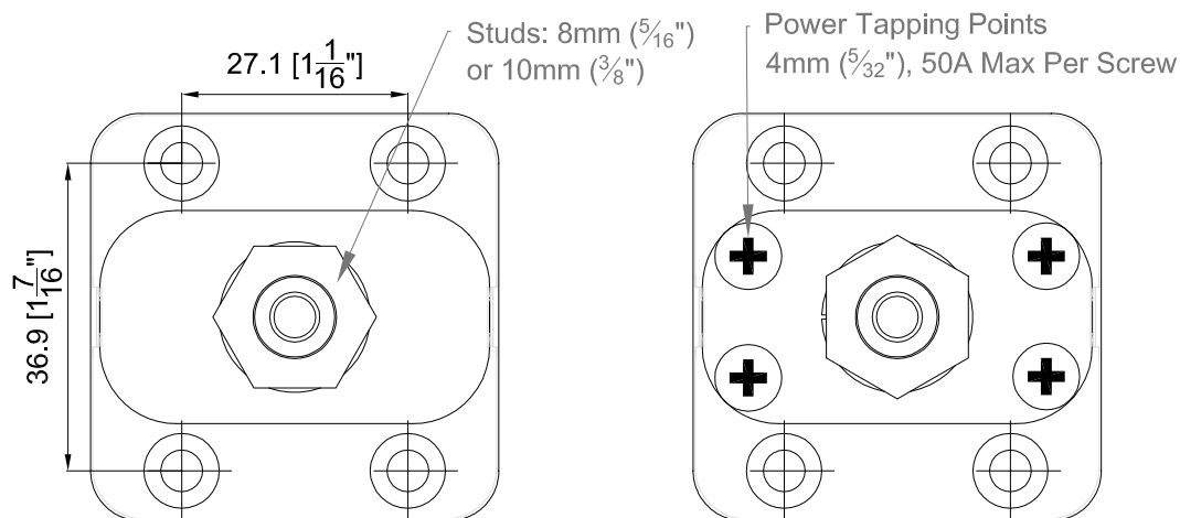
Single Studs With Power Tapping Plate, 8 & 10mm
